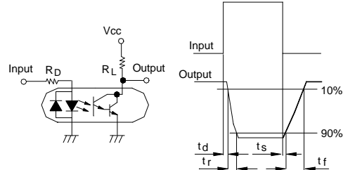
Test Circuit for Response Time
