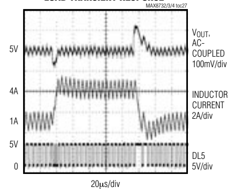
MAX8732/MAX8734 (TON = VCC) 5V PWM-MODE LOAD TRANSIENT RESPONSE
