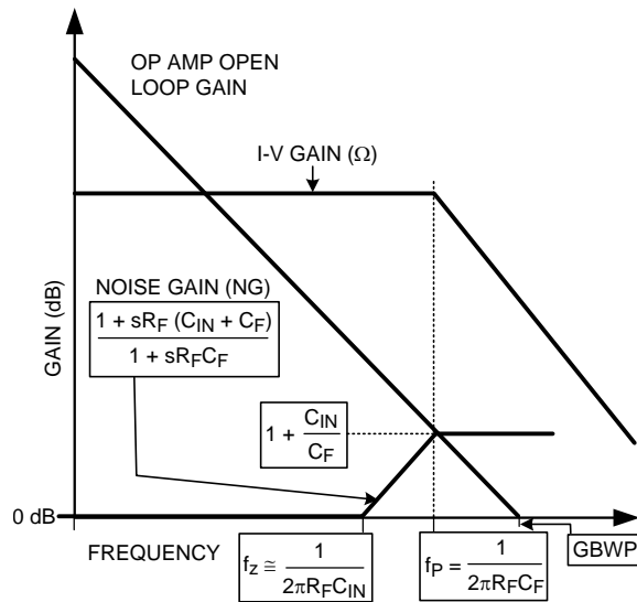
Figure 58. Transimpedance Amplifier Noise Gain and Transfer Function
