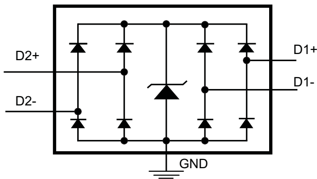
Figure 8. TPD4EUSB30 Circuit
