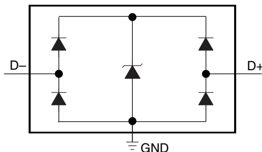
Figure 9. TPD2EUSB30/A Circuit
