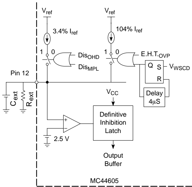
Figure 15. Disabling Block
