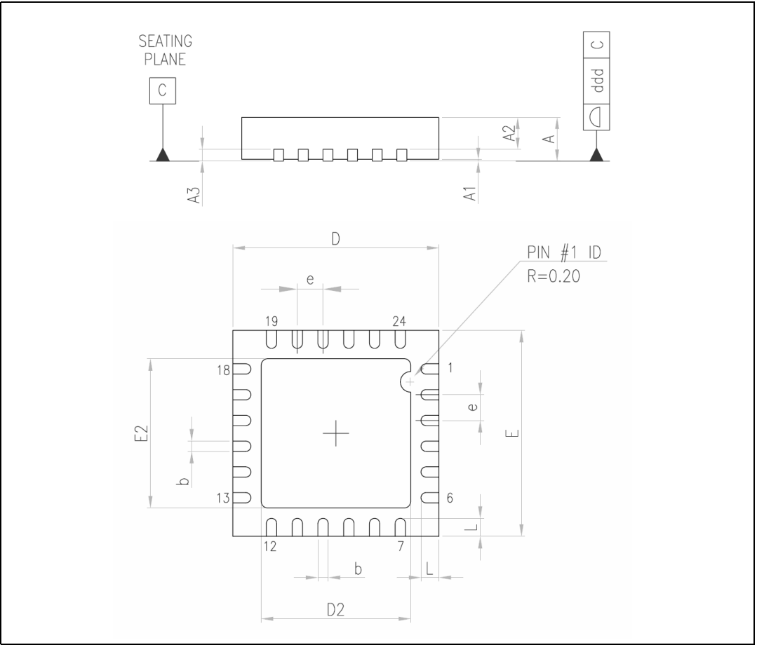
Figure 16. Package dimensions
