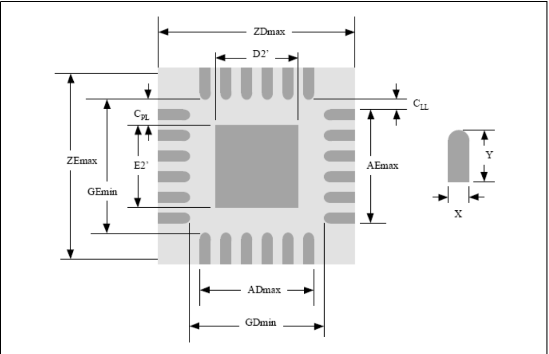
Figure 17. Footprint
