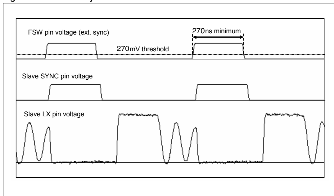
Figure 9. External sync waveforms
