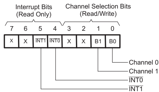
Figure 11. Control Register
