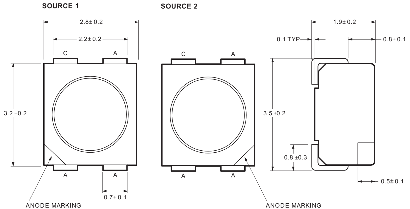
Figure 1: Package Drawing
