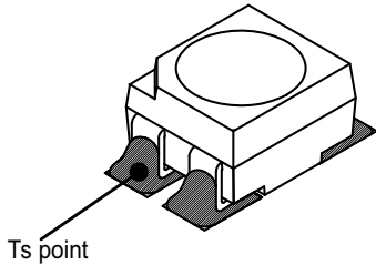
Figure 13: Solder Point Temperature on PCB
