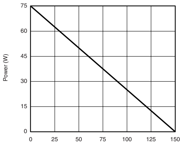
Power, Junction-to-Case
