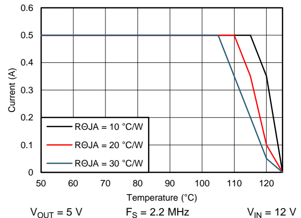
Figure 82. Derating Curve
