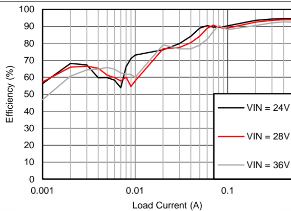
V_{OUT} = 12\text{ V} F_{SW} = 500\text{ kHz}
