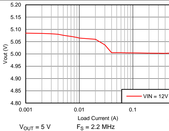
Figure 79. Output Voltage Regulation
