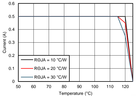
Figure 58. Derating Curve
